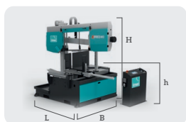
KS 652 NC B 1895 mm L 2870 mm H 2300 mm h 844 mm Kg 2100
