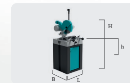
VELOX 350 B 610 mm L 880 mm H 990 mm h 895 mm Kg 163
