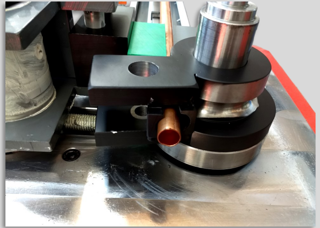
Eccentric clamp, front view
